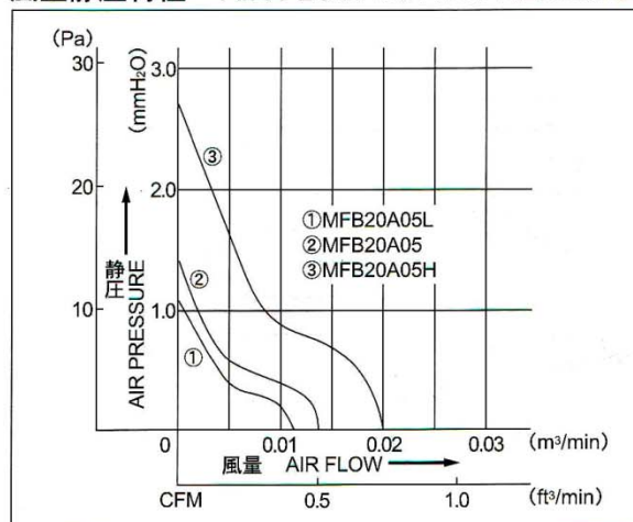
风量静压特性 AIR FLOW VS AIR PRESSURE
