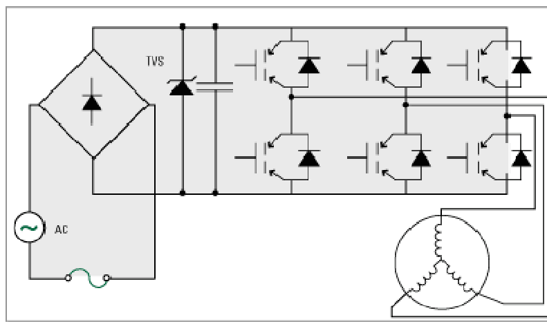
INVERTER DRIVE OVP/OCP
